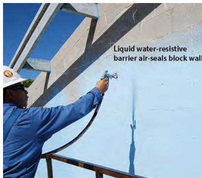
Liquid Water-Resistant Barrier: This retrofit serves two purposes: water proofing and air sealing.
