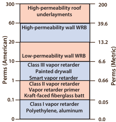
Vapor Permeability of Materials and Assemblies
