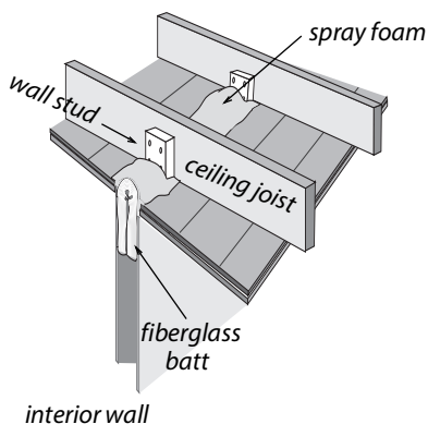
interior wall Balloon framed interior walls: Fiberglass insulation covered by a 1-inch layer of two-part foam seals wall cavities.
